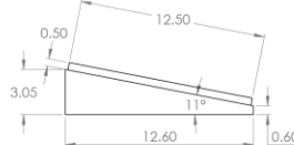
Mechanical Dimensions: Window with Wedge
