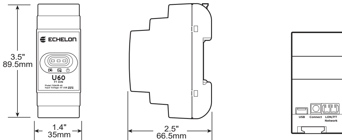
The U60 modules are designed for DIN-rail mounting; dimensions for both modules are the same
