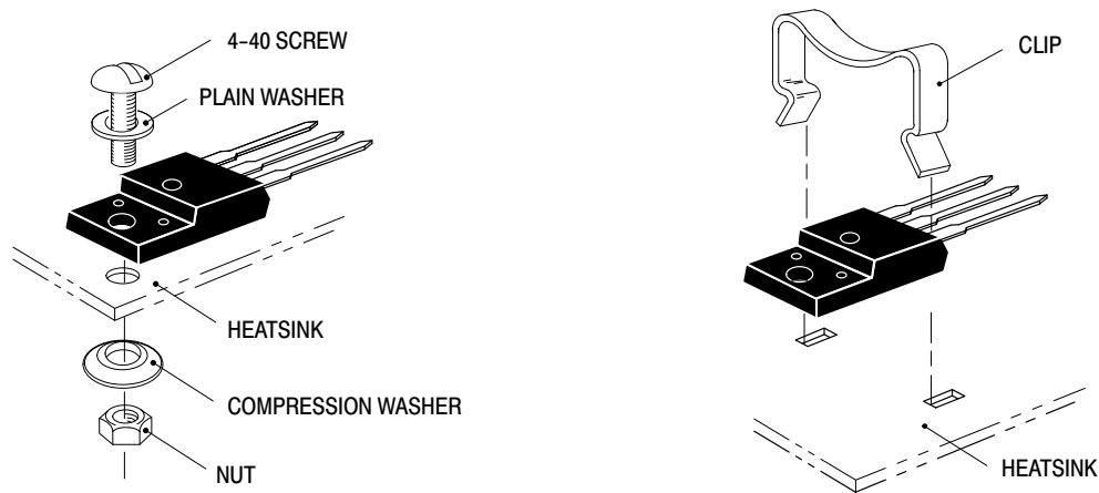
Figure 12. Typical Mounting Techniques*
