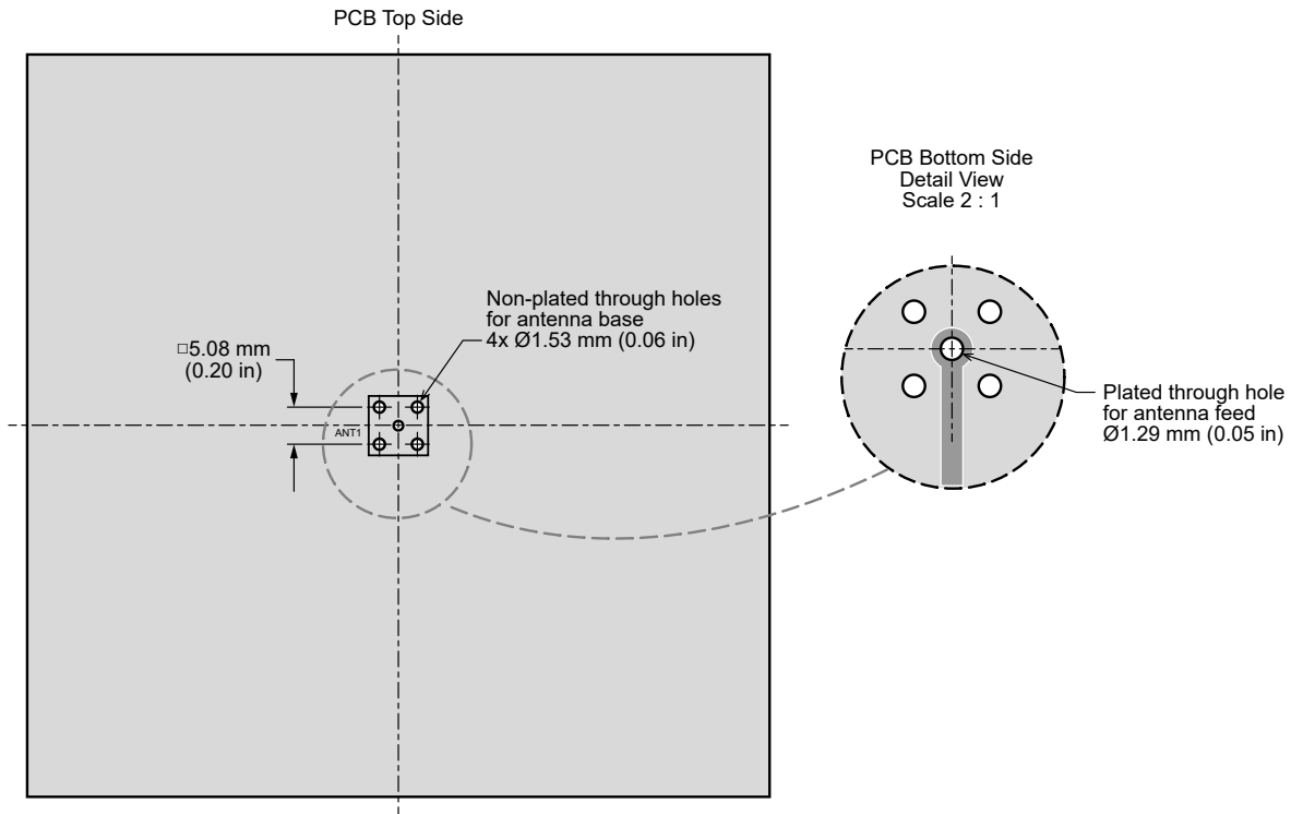
Figure 10. ANT-868-VHETH Antenna Placement on PCB
