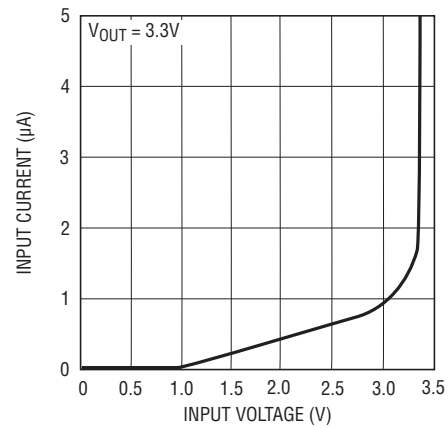
Figure 4. Input Current
