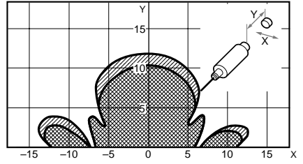
V600-D23P54 & V600-H52
