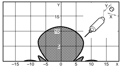
V600-D23P55 & V600-H52
