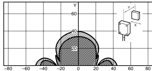
V600-D23P66SP & V600-H11
