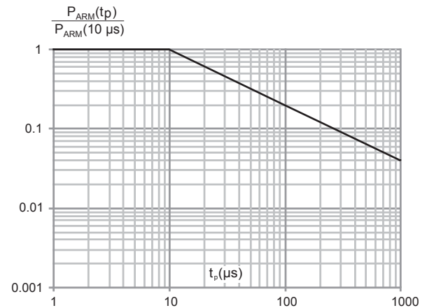
Figure 4. Normalized avalanche power derating versus pulse duration ( T_j = 125^{\circ}C )
