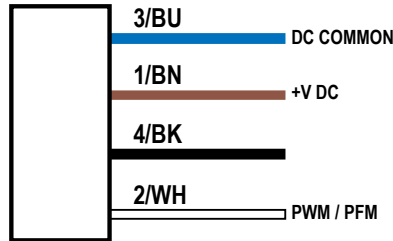
Figure 40. Wiring diagram for gauge
