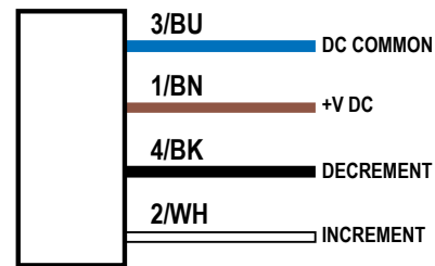
Figure 33. Wiring diagram for counter increment-decrement
