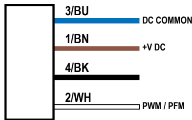
Figure 36. Wiring diagram for distance
