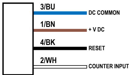
Figure 32. Wiring diagram for counter input
