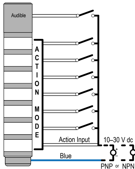
Figure 15. Wiring diagram for Action Input
