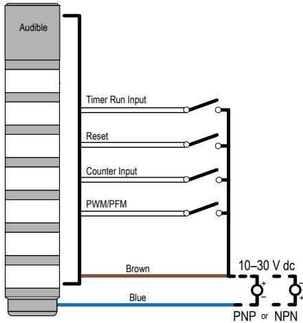
Figure 19. TL50 Pro wiring diagram for Advanced Mode
