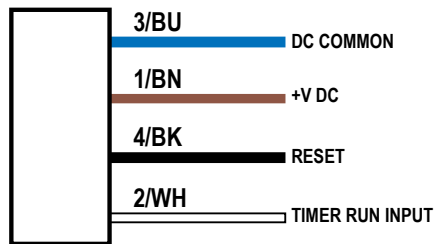
Figure 29. Wiring diagram for timer
