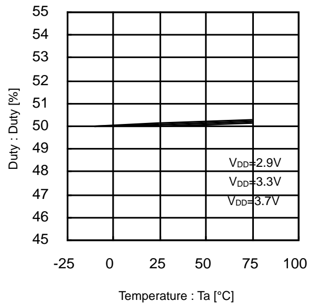
Figure 37. Duty vs Temperature (17.7MHz)
