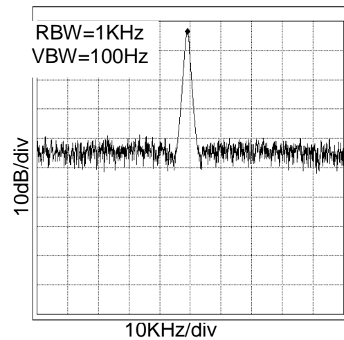
Figure 12. 98MHz Spectrum (At V_{DD}=3.3V and C_L=15pF )
