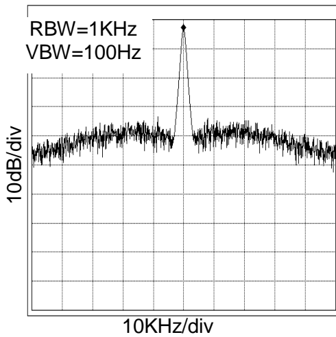
Figure 3. 135MHz Spectrum (At V_{DD}=3.3V and C_L=15pF )
