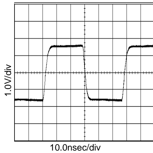
Figure 16. 17.7MHz Output Wave (At V_{DD}=3.3V and C_L=15pF )
