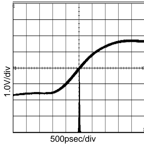
Figure 8. 108MHz Period-Jitter (At V_{DD}=3.3V and C_L=15pF )
