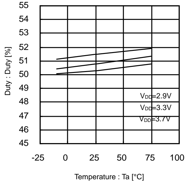
Figure 31. Duty vs Temperature (98MHz)
