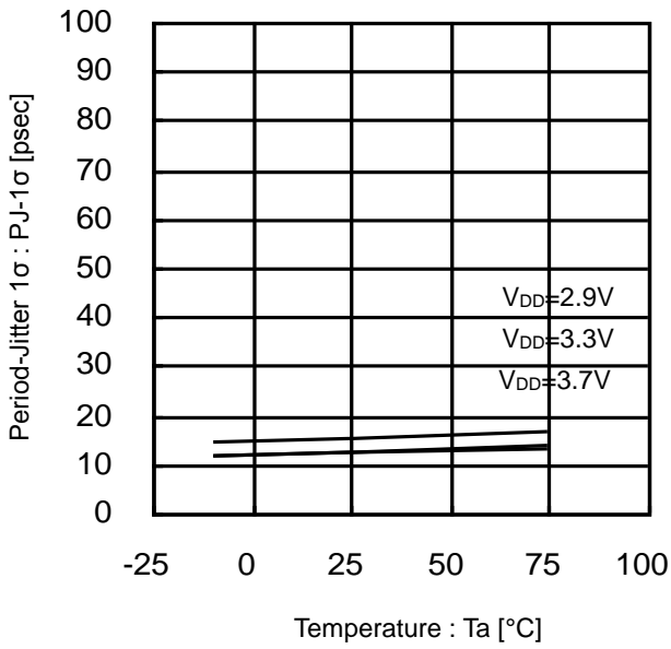
Figure 26. Period-Jitter 1σ vs Temperature (110MHz)
