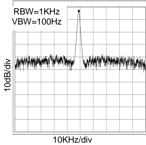
Figure 6. 110MHz Spectrum (At V_{DD}=3.3V and C_L=15pF )
