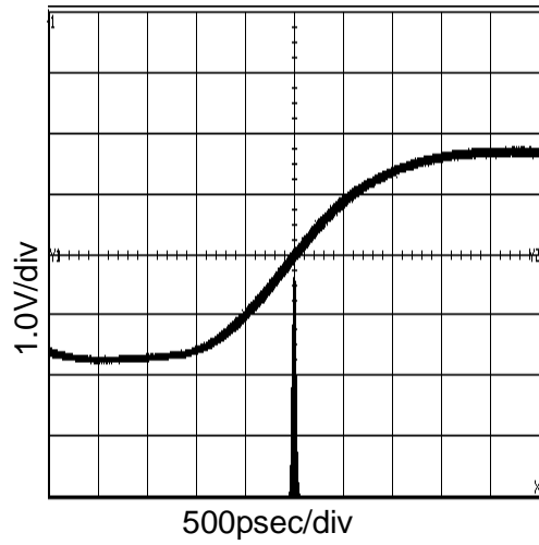
Figure 2. 135MHz Period-Jitter (At V_{DD}=3.3V and C_L=15pF )
