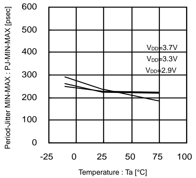
Figure 39. Period-Jitter MIN-MAX vs Temperature (17.7MHz)
