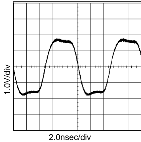
Figure 10. 98MHz Output Wave (At V_{DD}=3.3V and C_L=15pF )
