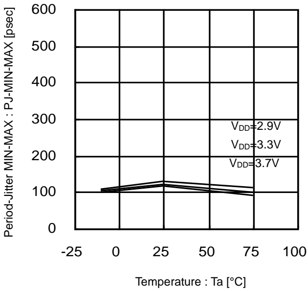
Figure 30. Period-Jitter MIN-MAX vs Temperature (108MHz)
