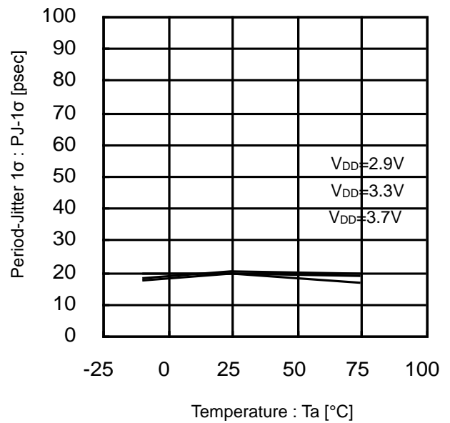
Figure 29. Period-Jitter 1σ vs Temperature (108MHz)
