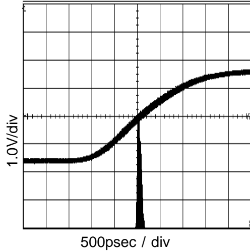
Figure 14. 48MHz Period-Jitter (At V_{DD}=3.3V and C_L=15pF )
