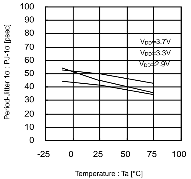
Figure 41. Period-Jitter 1σ vs Temperature (14.3MHz)
