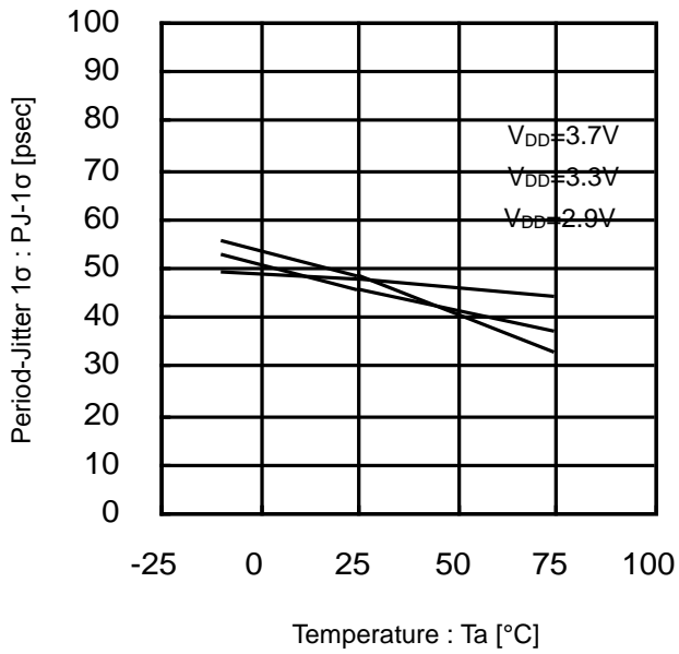
Figure 38. Period-Jitter 1σ vs Temperature (17.7MHz)
