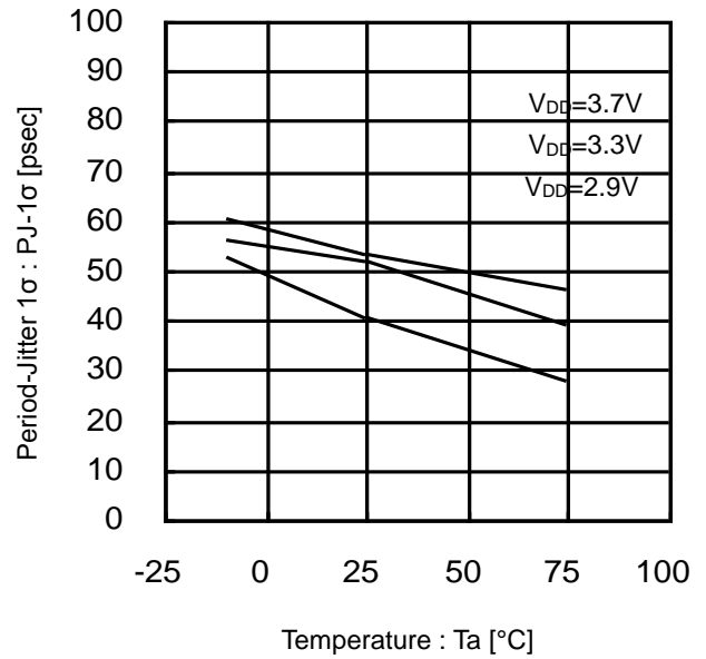
Figure 35. Period-Jitter 1σ vs Temperature (48MHz)
