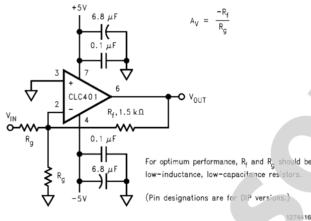
FIGURE 2. Recommended Inverting Gain Circuit
