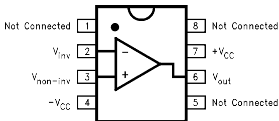
Pinout DIP & SOIC
