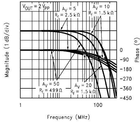
Non-Inverting Frequency Response 1274401
