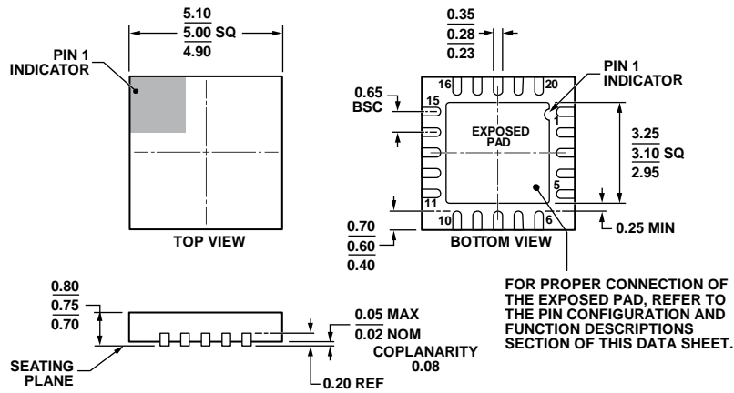
Figure 54. 20-Lead Lead Frame Chip Scale Package [LFCSP_WQ] 5 mm × 5 mm Body, Very Very Thin Quad (CP-20-9)
