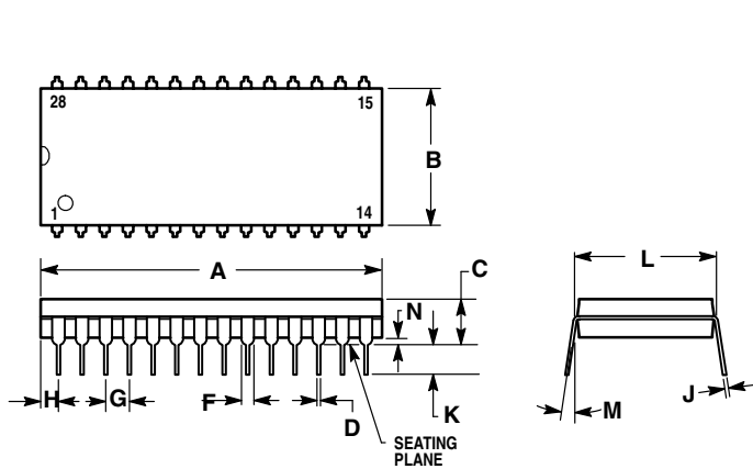
Figure 18-3. 28-Pin PDIP (Case #710)
