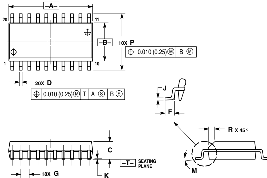
Figure 18-2. 20-Pin SOIC (Case #751D)
