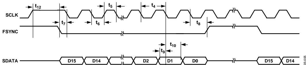
Figure 5. Serial Timing
