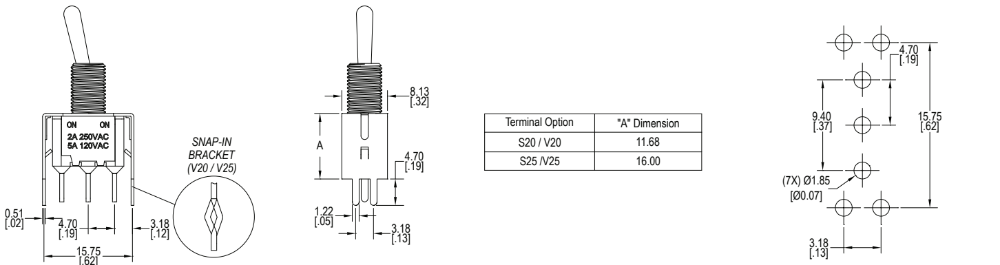
S20/S25 (V20/V25 - Snap-in) = PC pins with support bracket, single pole
