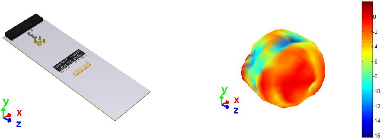
3D pattern at 2600MHz
