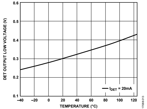
Figure 14. DET Output Low Voltage vs. Temperature
