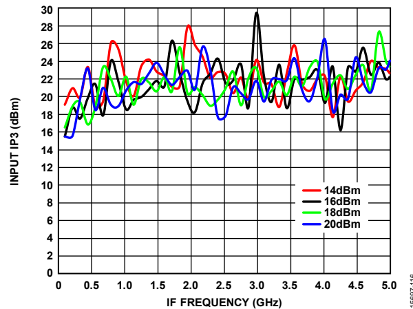
Figure 116. Input IP3 vs. IF Frequency at Various LO Drives, LO Frequency = 32 GHz, T A = 25°C
