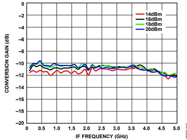
Figure 115. Conversion Gain vs. IF Frequency at Various LO Drives, LO Frequency = 32 GHz, T A = 25°C
