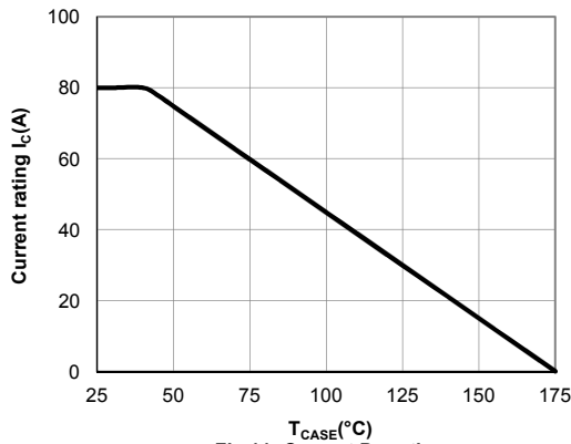
Fig 11: Current De-rating
