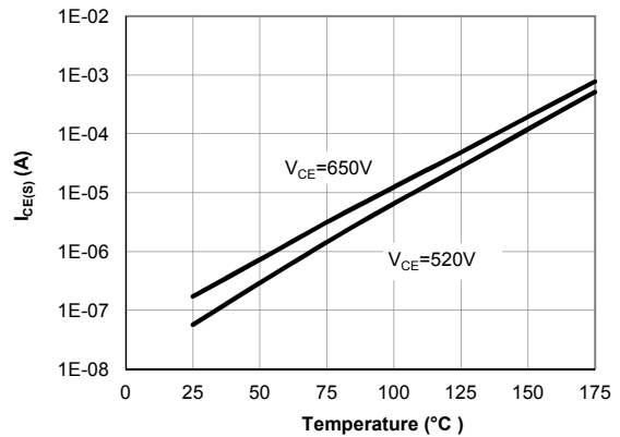
Fig 12: Diode Reverse Leakage Current vs. Junction Temperature
