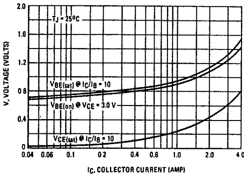
FIGURE 9 - "ON" VOLTAGES
