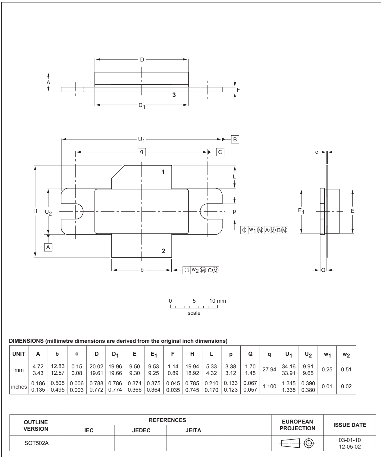
Fig 15. Package outline SOT502A
