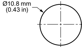
Figure 2. ANT-868-WRT Series Antenna Recommended Enclosure Mounting Dimensions
