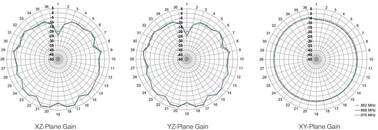
Figure 17. ANT-868-WRT Radiation Patterns, Center of Ground Plane
