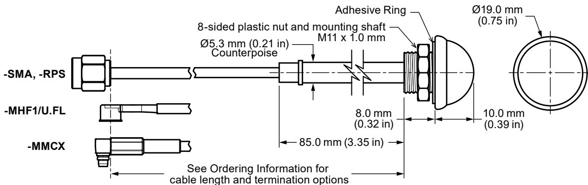
Figure 1. ANT-868-WRT Antenna Dimensions
