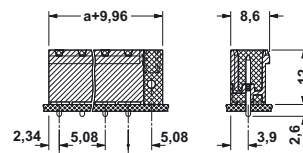
CCV 2,5/...-GFL-5,08P26THR
