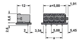
CCA 2,5/...-GR-5,08RNP26THR
