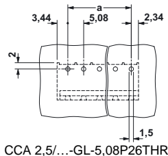
CCA 2,5/...-GL-5,08P26THR
