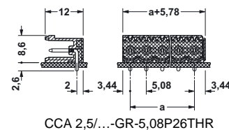
CCA 2,5/...-GR-5,08P26THR
