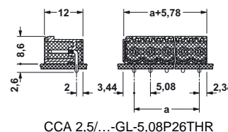
CCA 2,5/...-GL-5,08P26THR
