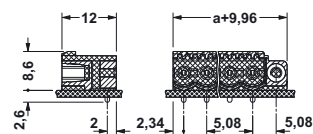
CC 2,5/...-GFR-5,08P26THR
