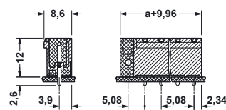
CCV 2,5/...-GFR-5,08P26THR
