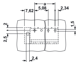
CC 2,5/...-GFL-5,08P26THR
