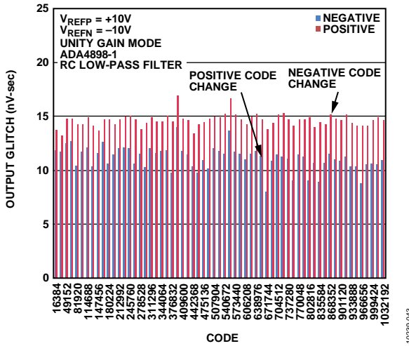
Figure 42. 6 MSB Segment Glitch Energy for \pm 10 V_{REF}
