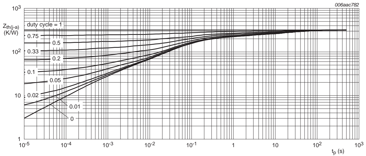
Fig 3. Transient thermal impedance from junction to ambient as a function of pulse duration for PDTA143XM (SOT883); typical values
