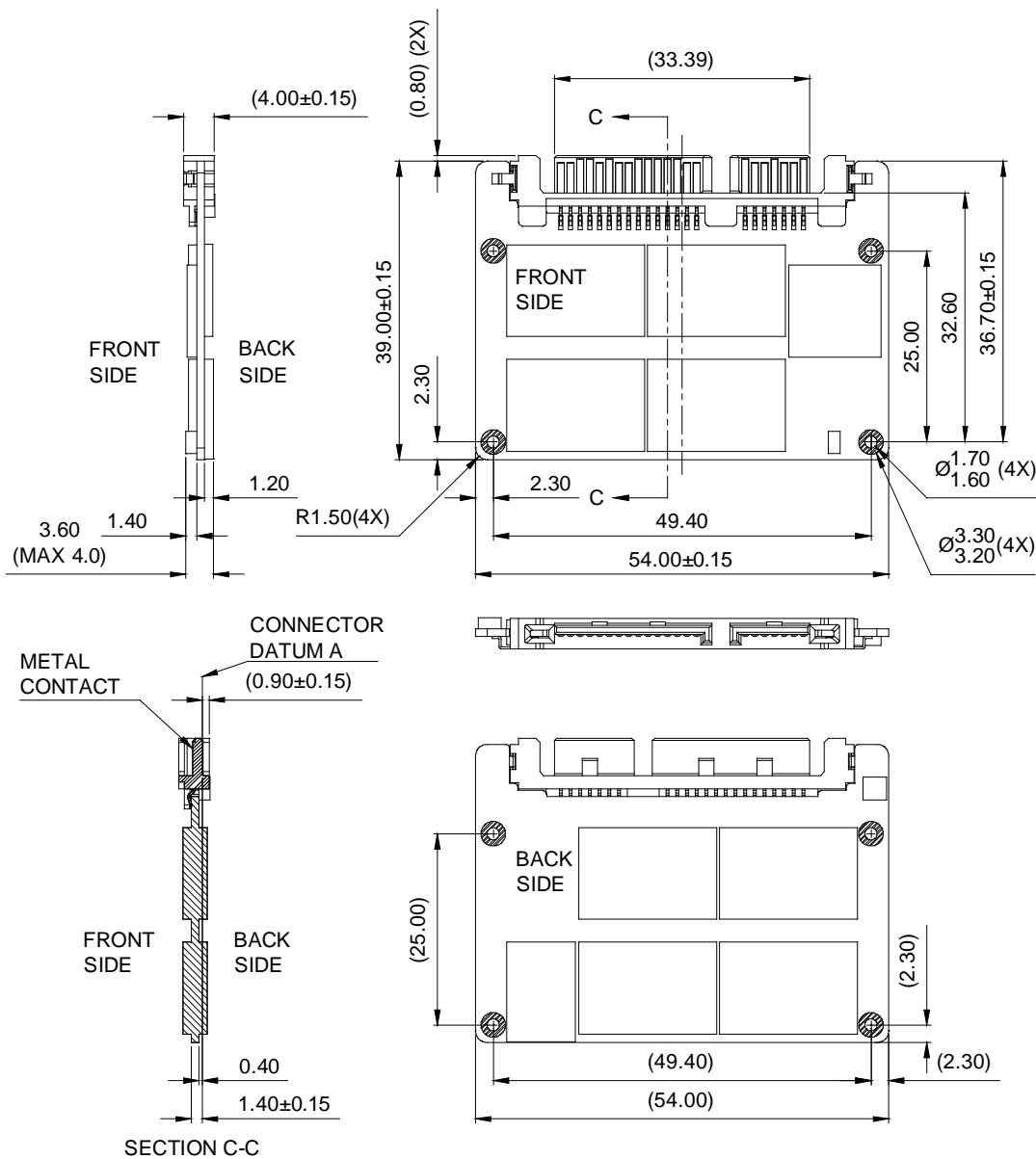
Figure 2: Mechanical Dimensions
