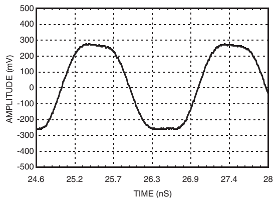
Output Voltage Waveform, Pin= 0 dBm, Fout= 500 MHz, T= 25 °C
