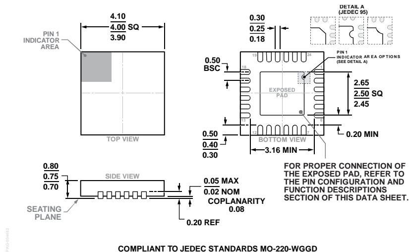
Figure 76. 24-Lead Lead Frame Chip Scale Package [LFCSP] 4 mm × 4 mm Body and 0.75 mm Package Height (CP-24-7)
