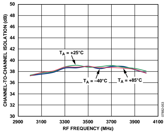
Figure 53. Channel-to-Channel Isolation
