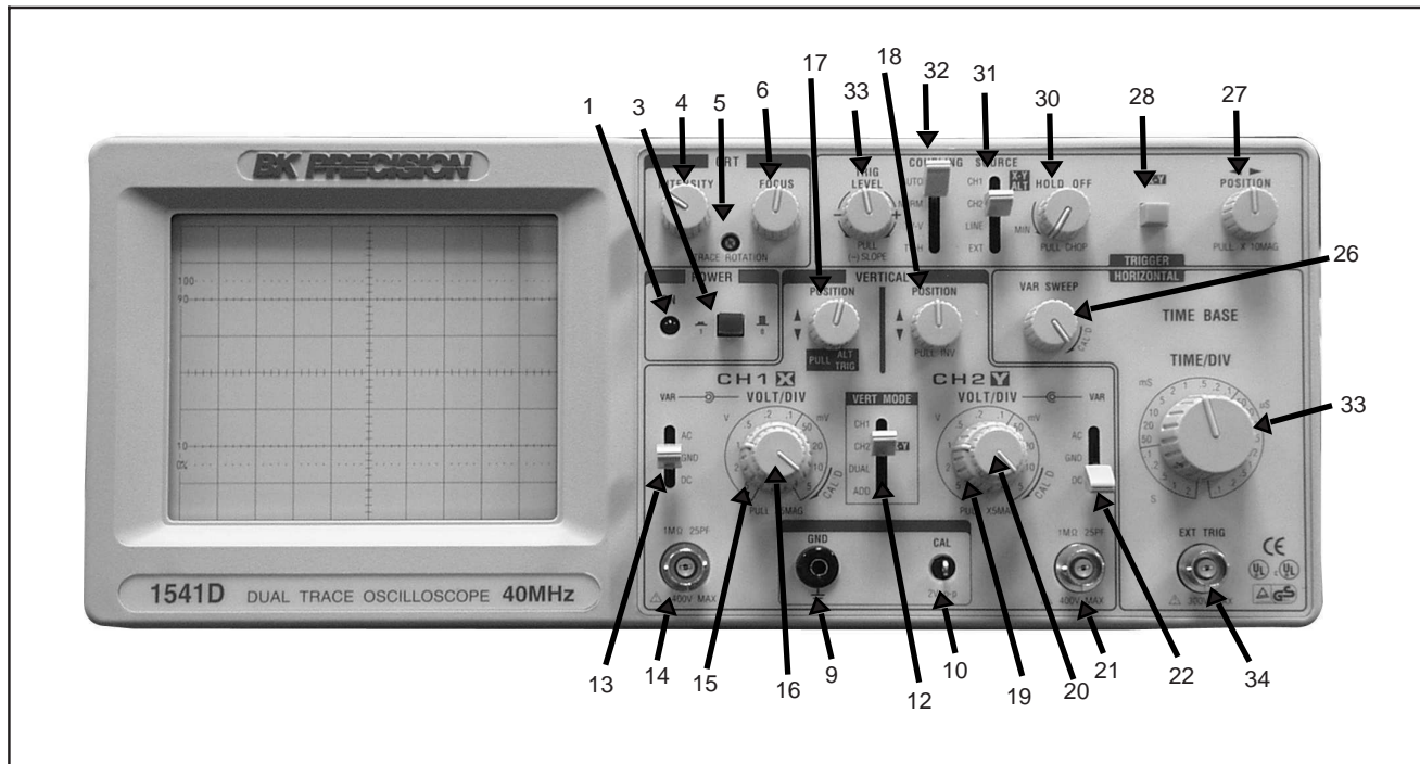
Fig. 2. Model 1541D Controls and Indicators.
