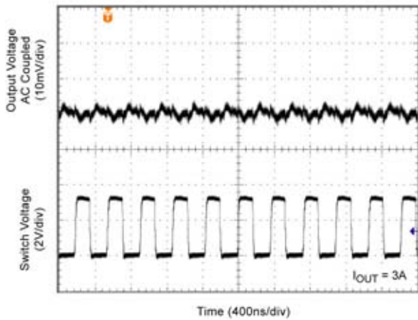
Output Ripple
