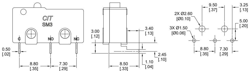
Right Angle PC Terminals
