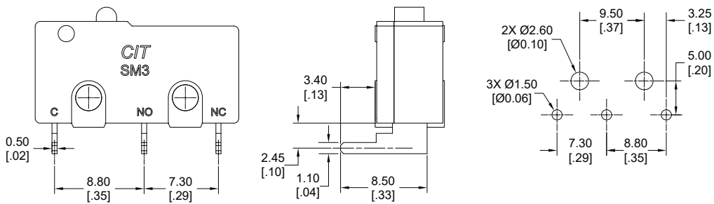
Left Angle PC Terminals
