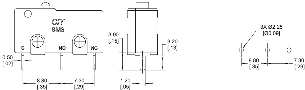
PC Terminals
