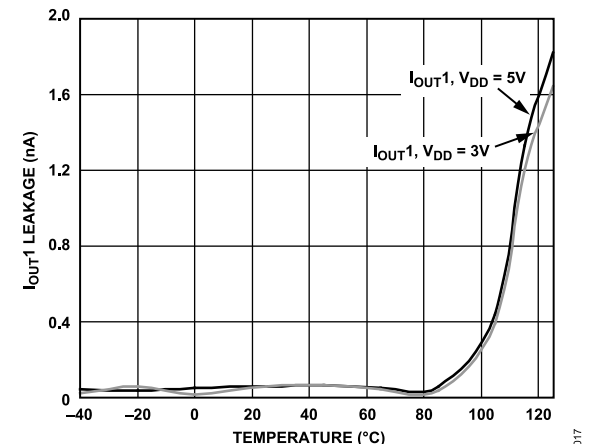
Figure 17. IOUT1 Leakage Current vs. Temperature
