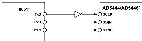
Figure 49. 80C51/80L51 to AD5444/AD5446 Interface
