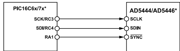
Figure 52. PIC16C6x/7x to AD5444/AD5446 Interface
