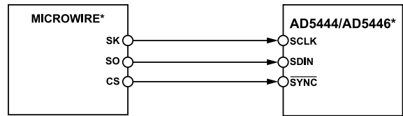
Figure 51. MICROWIRE to AD5444/AD5446 Interface
