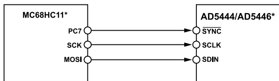
Figure 50. MC68HC11 to AD5444/AD5446 Interface
