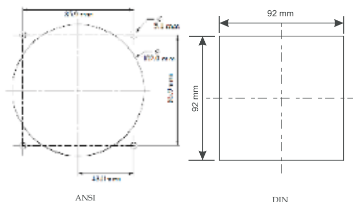
PANEL CUTOUT
