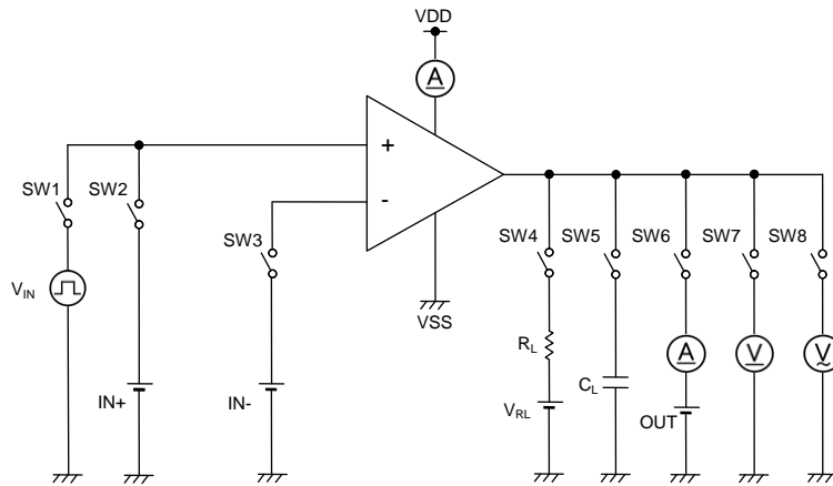
Figure 42. Test Circuit 2
