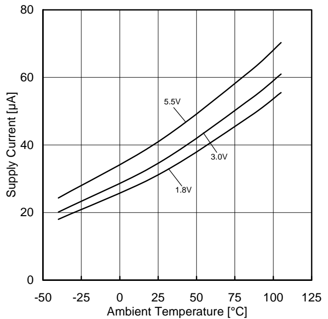
Figure 24. Supply Current vs Ambient Temperature
