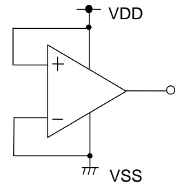
Figure 45. Example of Application Circuit for Unused Comparator
