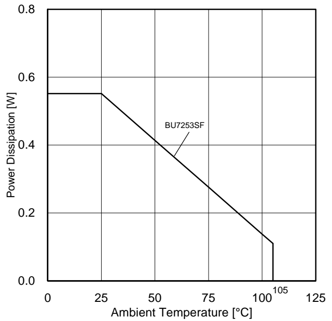
Figure 22. Power Dissipation vs Ambient Temperature (Derating Curve)
