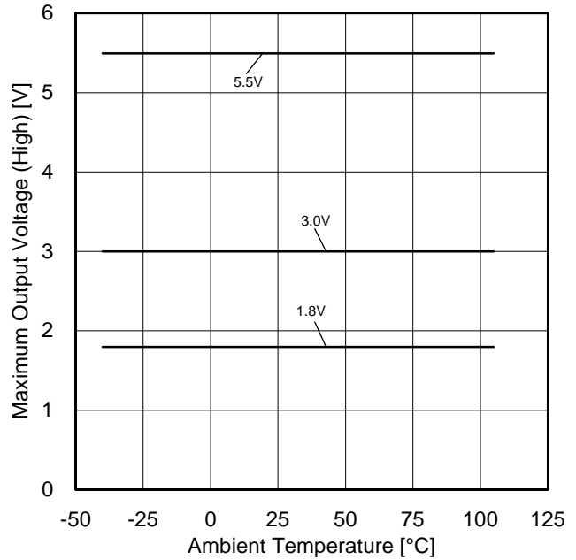
Figure 26. Maximum Output Voltage (High) vs Ambient Temperature ( R_L=10k\Omega )
