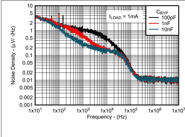
Figure 6-31. Output Noise Density vs Frequency for New Chip
