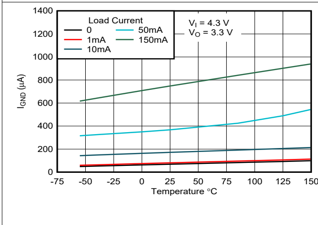
Figure 6-35. Ground-Pin Current vs Temperature for New Chip
