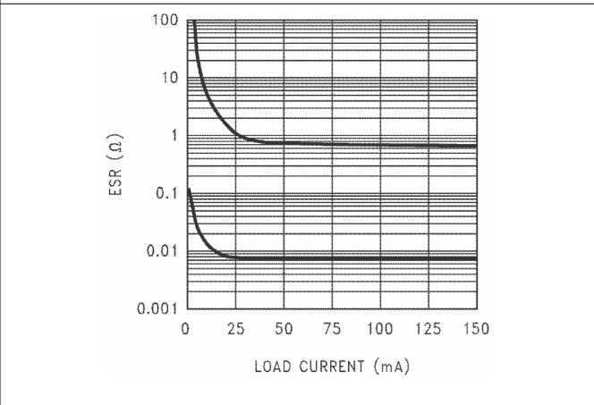
Figure 6-36. 2.2-µF Stable ESR Range for Output Voltage ≤ 2.3 V for Legacy Chip
