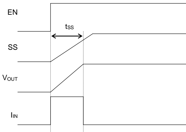
(1) Soft Start Function
