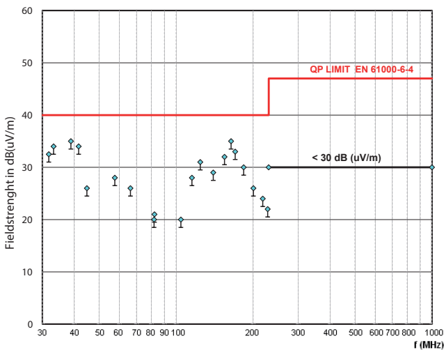
Fig. 9a XRCM60-24: Typ. radiated disturbances in 10 m distance ( V_i = 16.8 V, I_{i\text{nom}} , resistive load, quasi peak).
