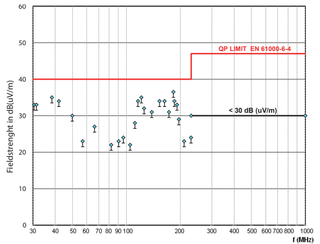
Fig. 9b XRCM60-24: Typ. radiated disturbances in 10 m distance ( V_i = 137.5 V, I_{i\text{nom}} , resistive load, quasi peak).
