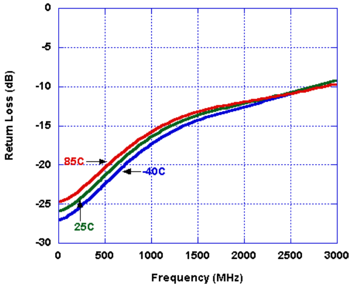
Figure 7. RF1 Return Loss (Switch = ON)
