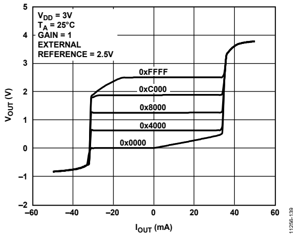
Figure 33. Source and Sink Capability at 3 V, Gain = 1
