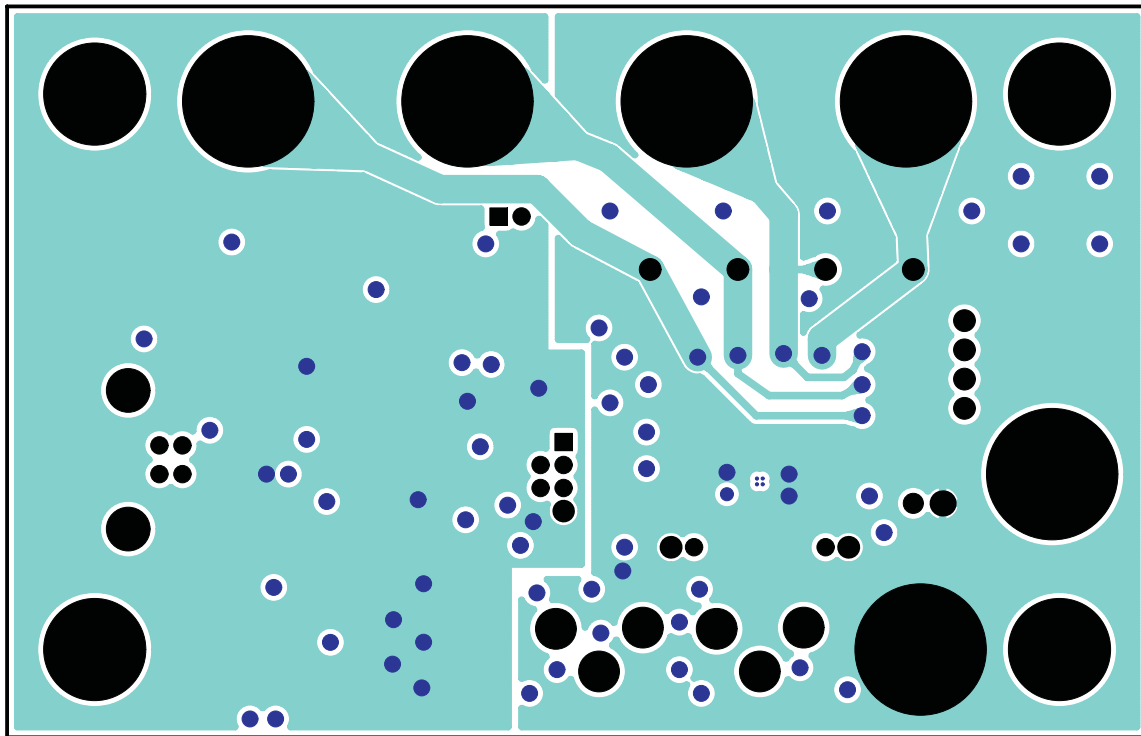
Figure 9. TPA2016D2EVM – Layer 3
