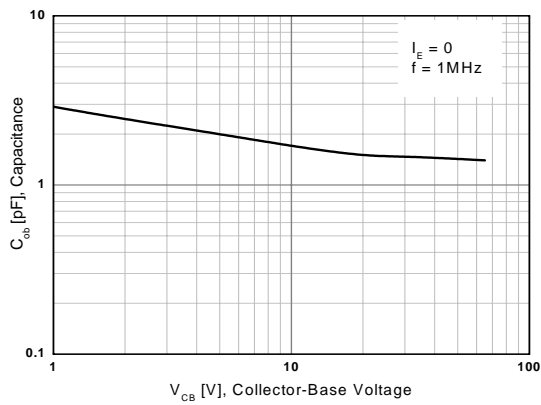
Figure 5. Output Capacitance
