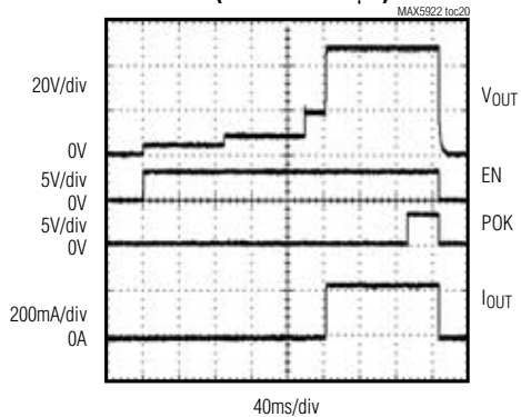
STARTUP WITH VALID PD (25kΩ AND 0.1μF)
