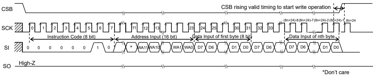
Figure 42. Write Command (Byte Write)
