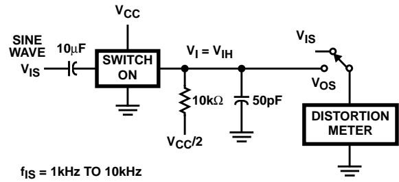
f_{IS} = 1\text{kHz TO } 10\text{kHz} FIGURE 10. TOTAL HARMONIC DISTORTION TEST CIRCUIT
