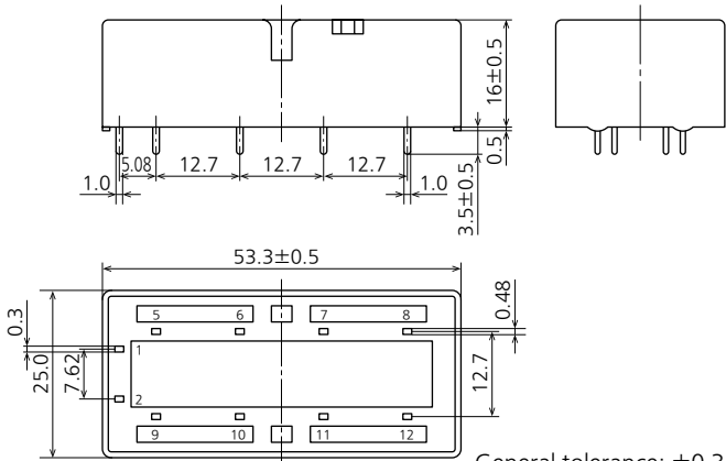
External dimensions
