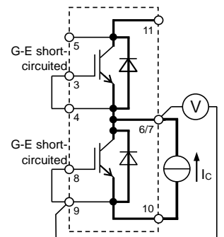
Di1 V EC characteristics test circuit
