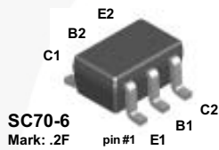
Figure 1. FFB2907A Device Package
