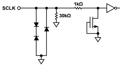
Figure 33. Equivalent SCLK Input Circuit
