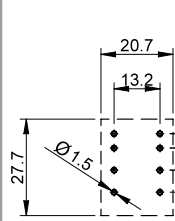
Copper side view
