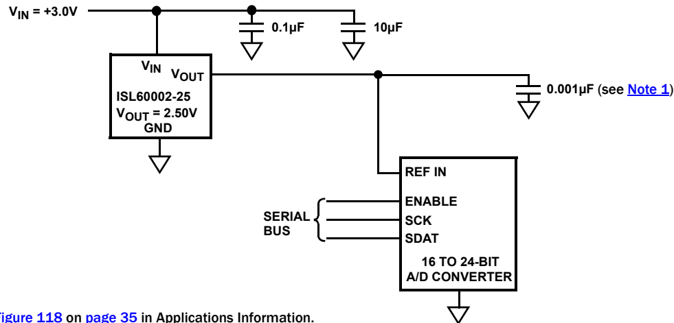
FIGURE 1. TYPICAL APPLICATION
