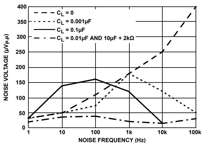
FIGURE 117. NOISE REDUCTION
