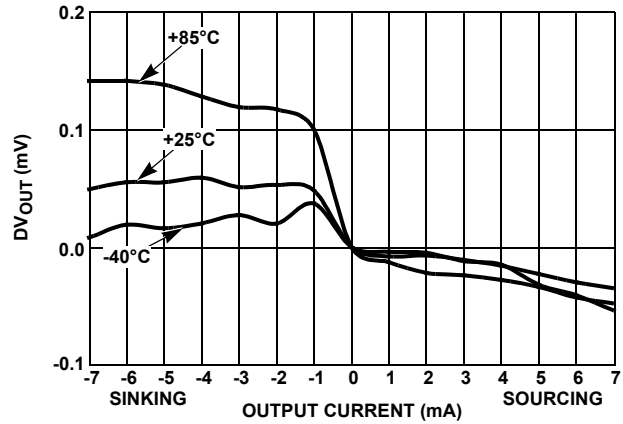
FIGURE 77. LOAD REGULATION OVER-TEMPERATURE
