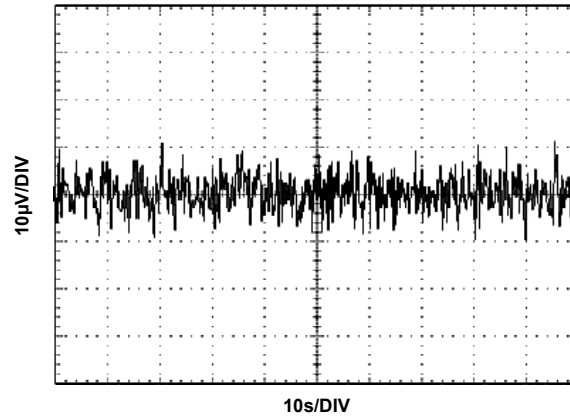
FIGURE 41. V_{OUT} NOISE
