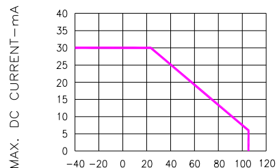
Fig.6 MAX. ALLOWABLE DC CURRENT VS. AMBIENT TEMPERATURE
